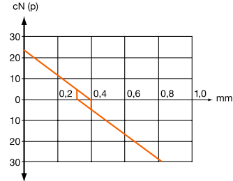
Contact force/travel
